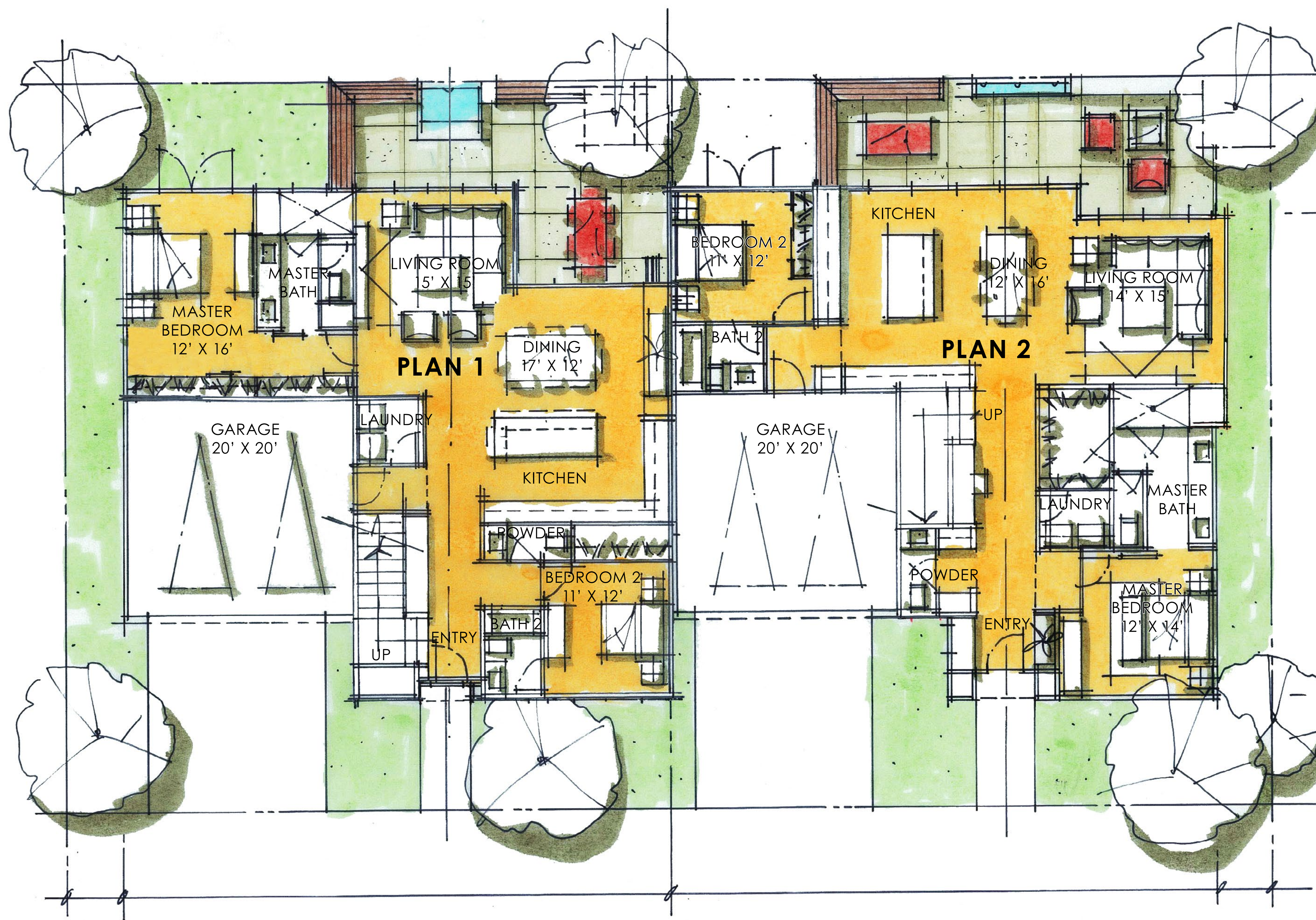
FIRST FLOOR
